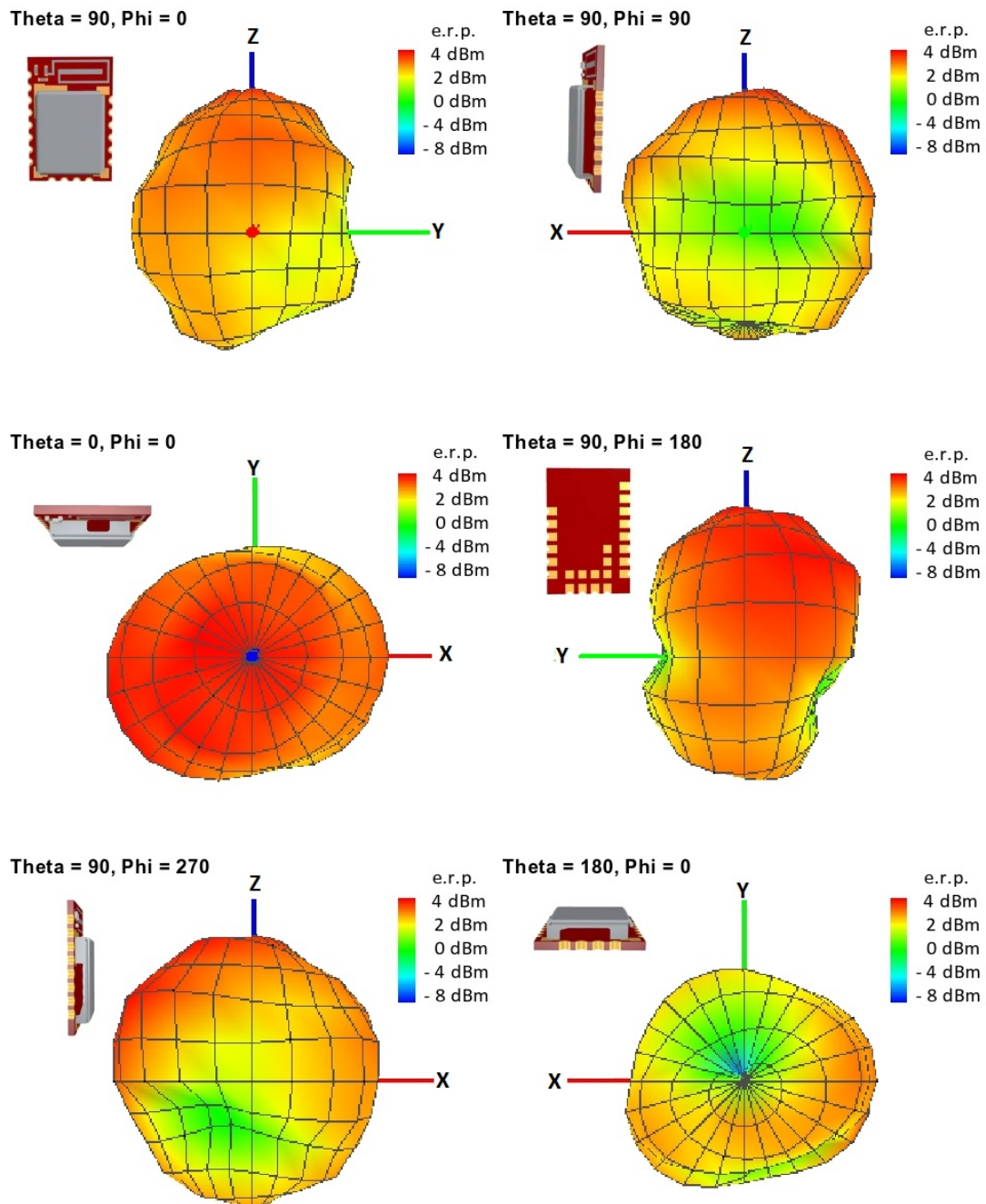
Figure 13: Antenna characteristic from integrated antenna measured on official evaluation board 1
